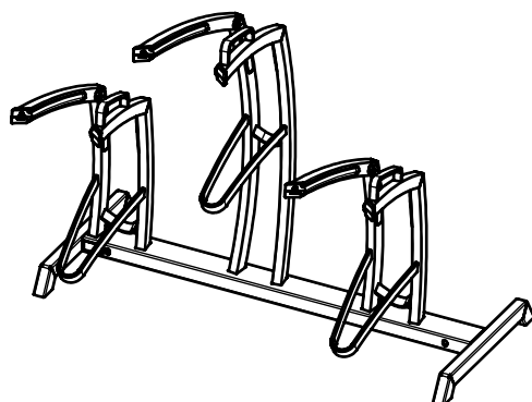
Griffin 375-3 single sided assembly 30635000
